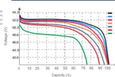
Different Temperature Discharge Curve(0.2C)
