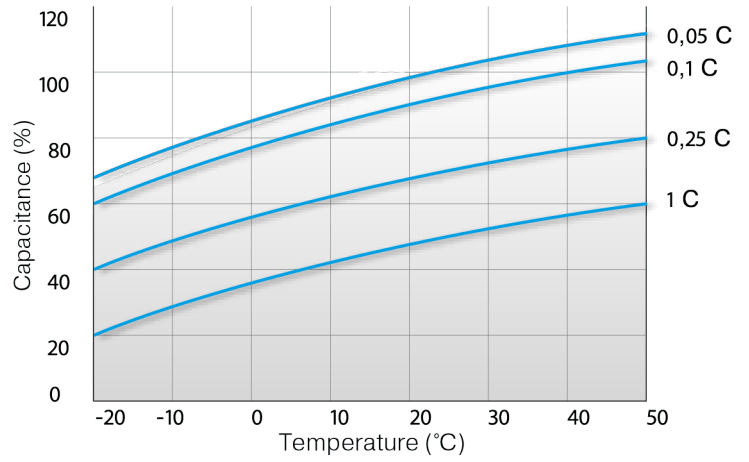
TEMPERATURE INFLUENCE ON THE CAPACITANCE
