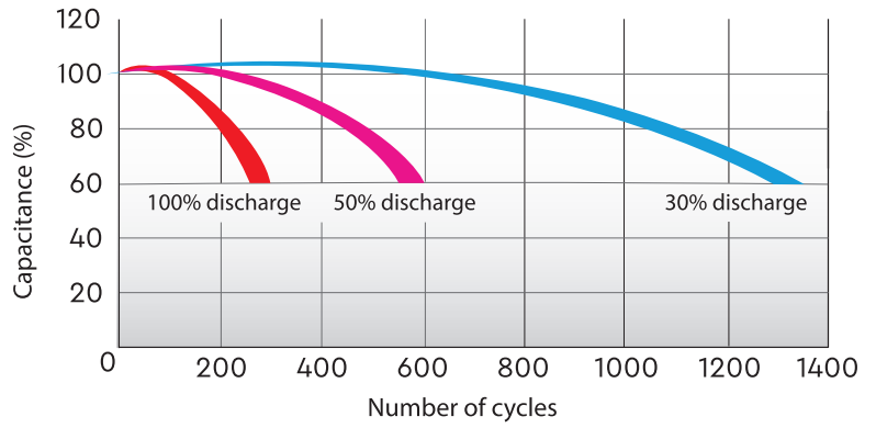
SERVICE LIFE IN CYCLIC MODE (Over 65 Ah)
