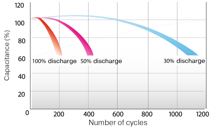
SERVICE LIFE IN BUFFER MODE (5 YEARS)
