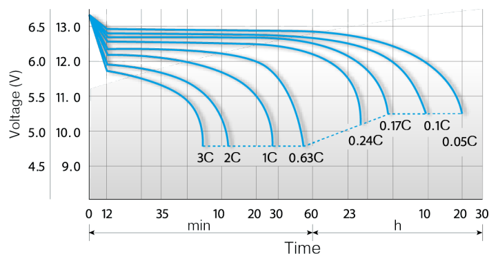
DISCHARGE CHARACTERISTICS
