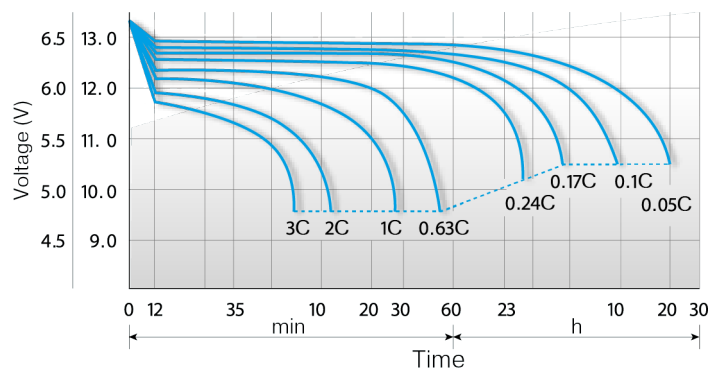
DISCHARGE CHARACTERISTICS
